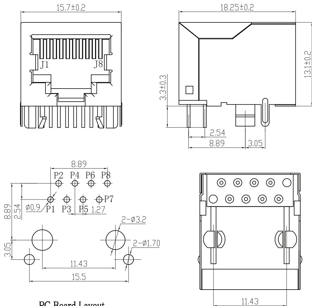
PC Board Layout
