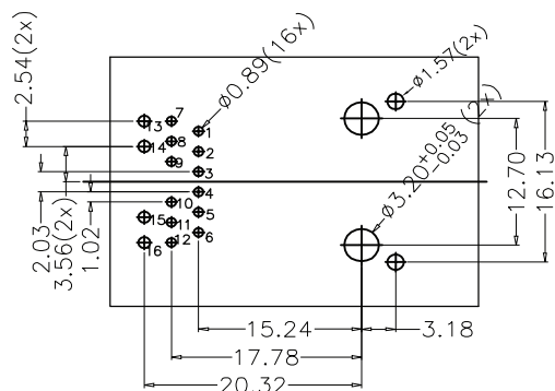
Recommend P.C.B Layout viewed From Component Side
